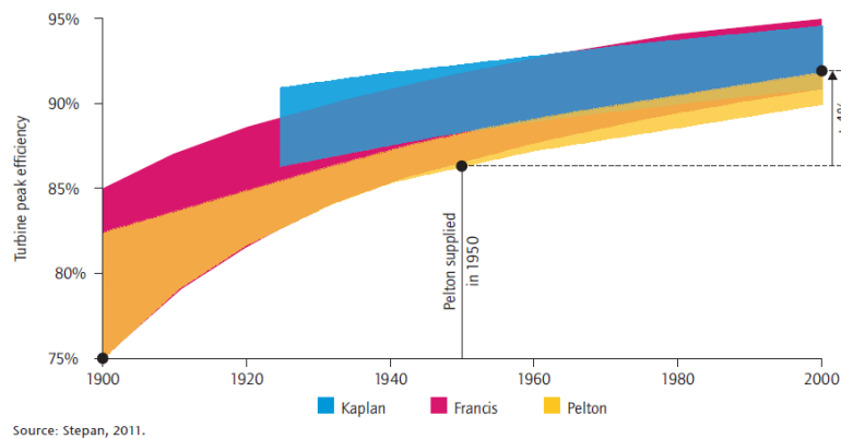
Improvement of hydraulic performance over time (ref. 8)
